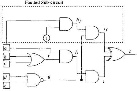
(b) ATPG circuit example
